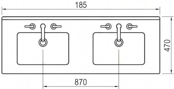
Top-Down Plan.
