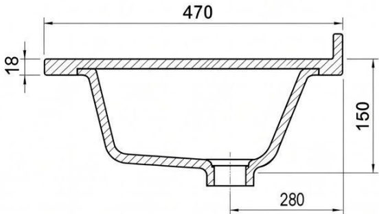
Sectional Profile
