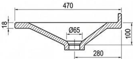
Sectional Profile
