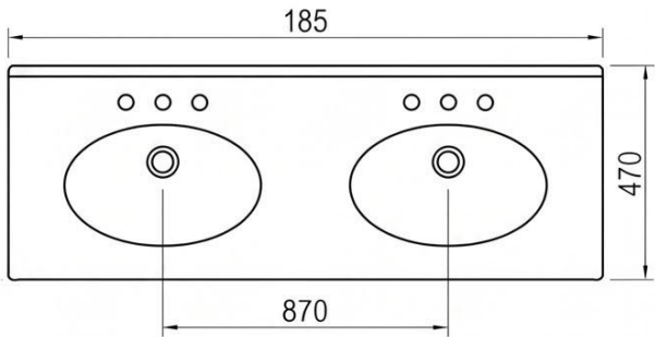
Top-Down Plan.
