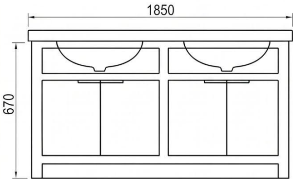
Front Elevation
