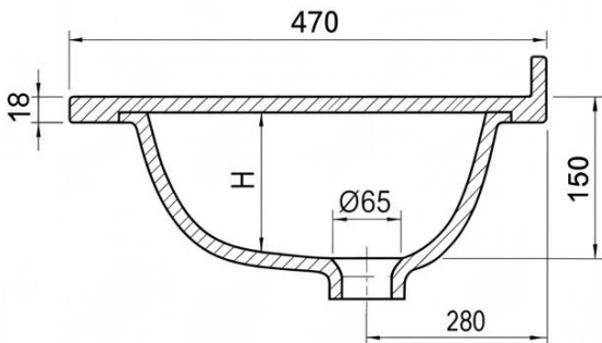
Sectional Profile
