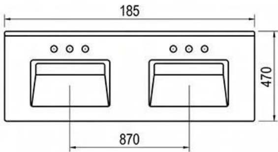
Top-Down Plan.
